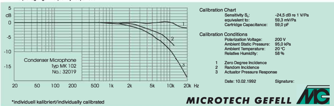
Frequenzgänge/Frequency responses
